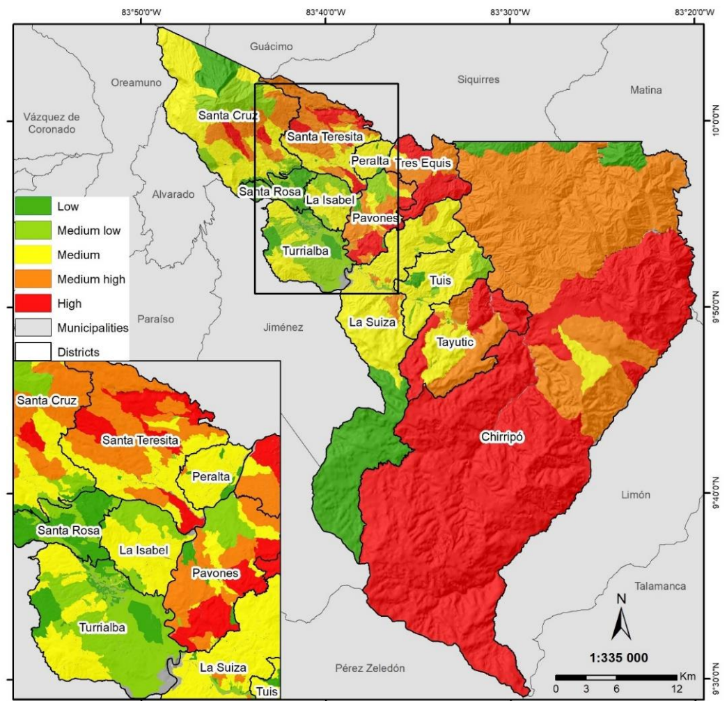
Figure 8. Exposure-factored extreme rainfall risk index for the Turrialba municipality.
