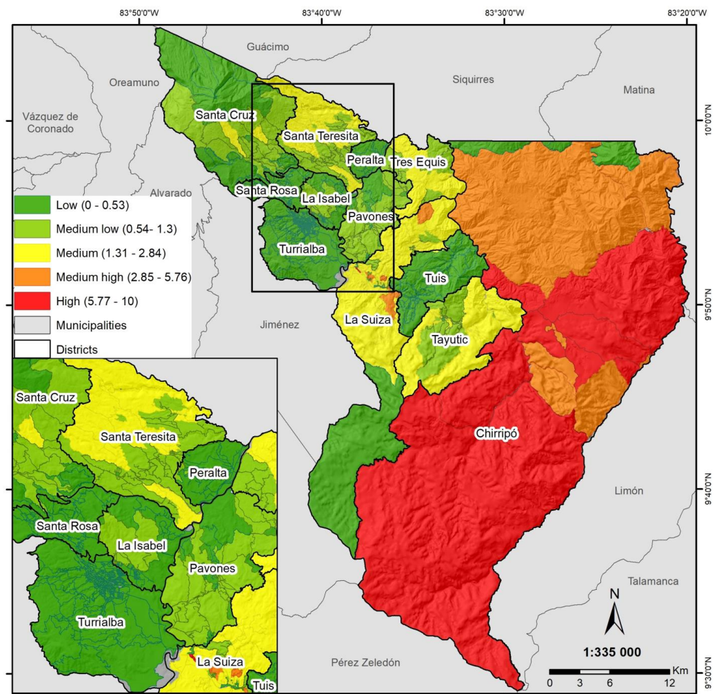
Figure 6. Extreme rainfall risk index for the Turrialba municipality.
