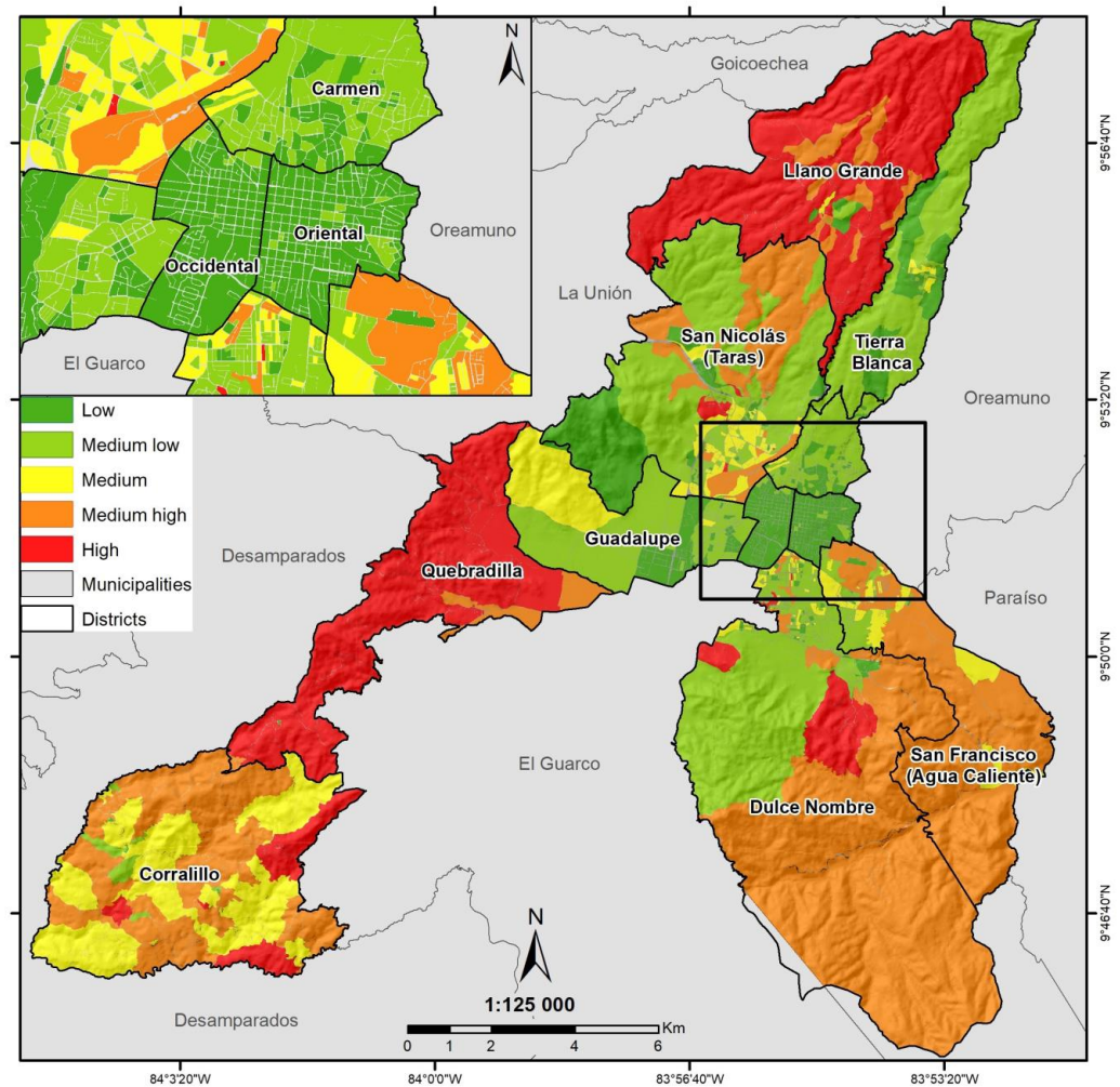
Figure 5. Exposure-factored extreme rainfall risk index for the Cartago municipality.
