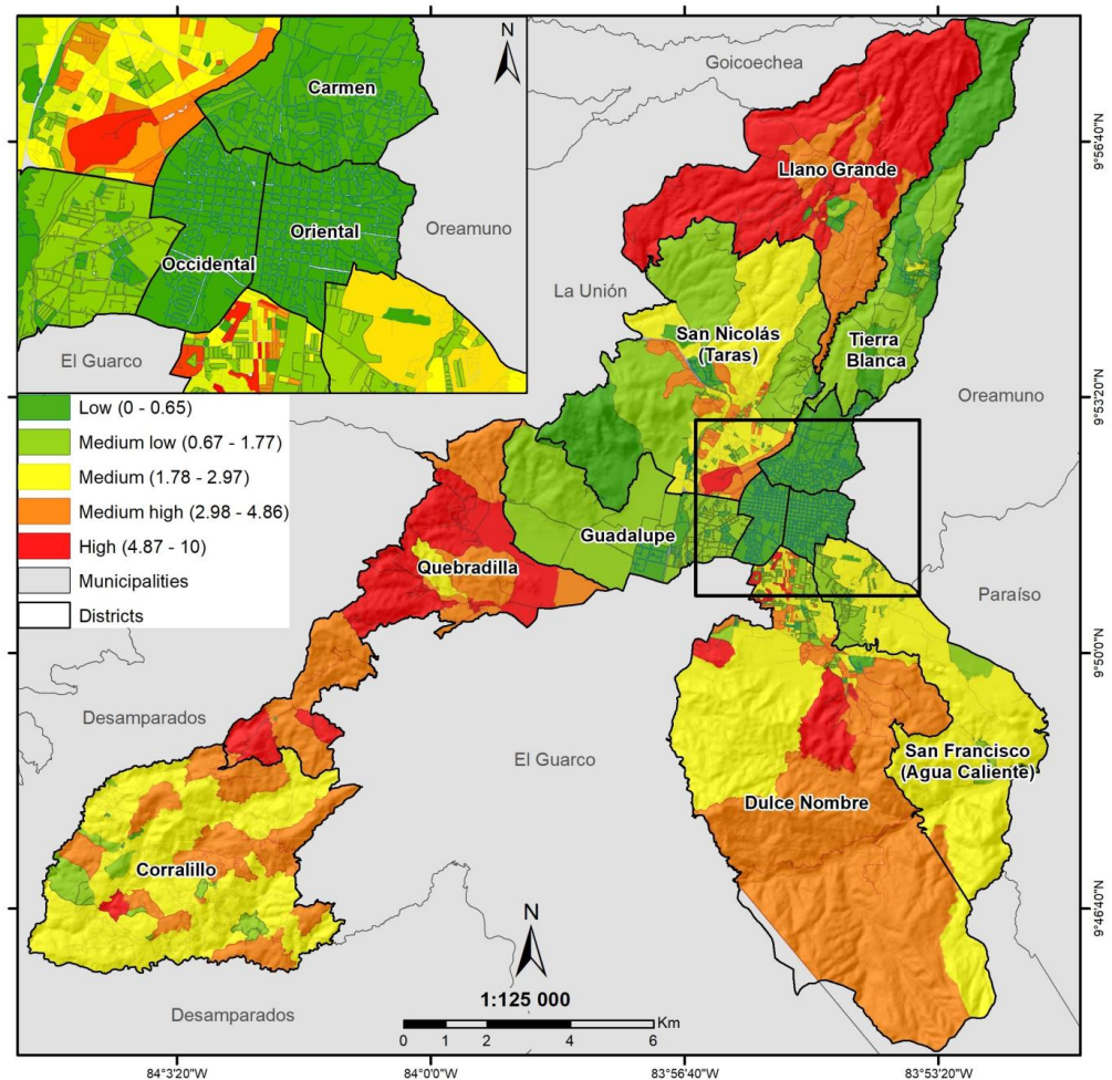
Figure 3. Extreme rainfall risk index for the Cartago municipality.
