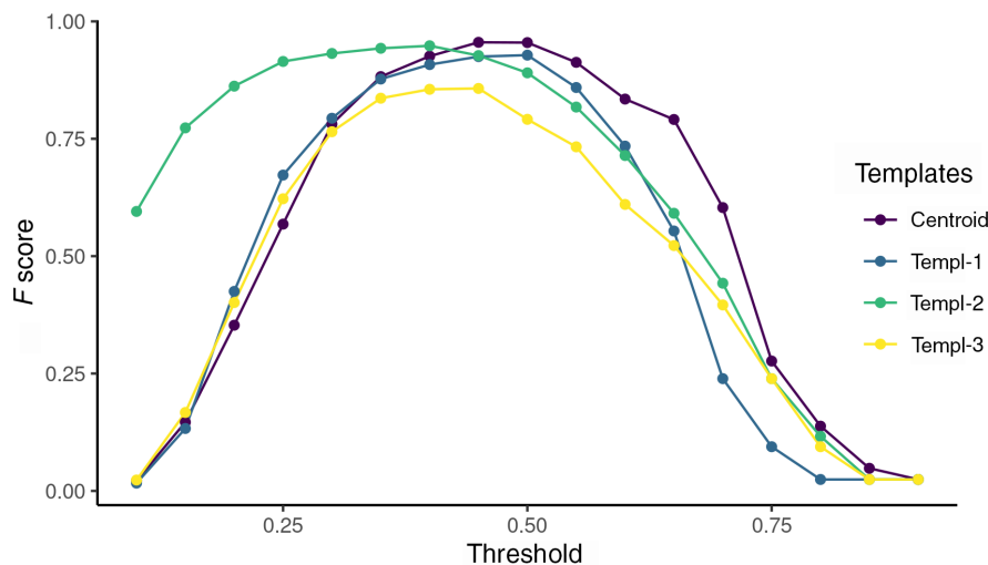
FIGURE 3 Changes in F score across the range of cross-correlation threshold values for four sound templates.
