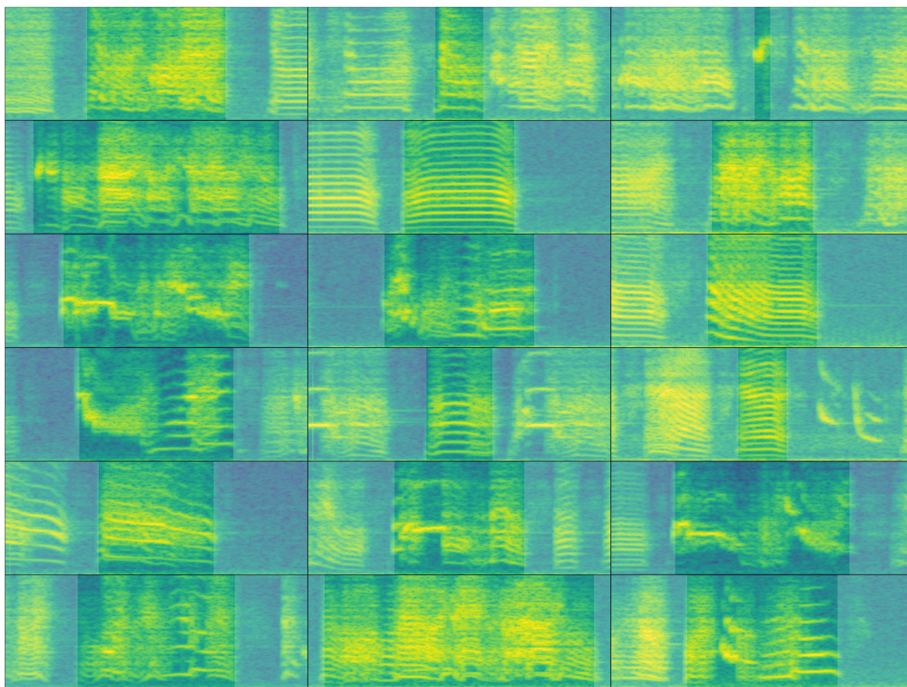
FIGURE 4 Example spectrograms of male zebra finch songs for each of the 18 sound files used in the analysis. The highest signal-to-noise ratio call by sound file are shown. The time scale range is 359 ms and the frequency range 0–11 kHz. Signals have been highlighted for visualization purposes only.
