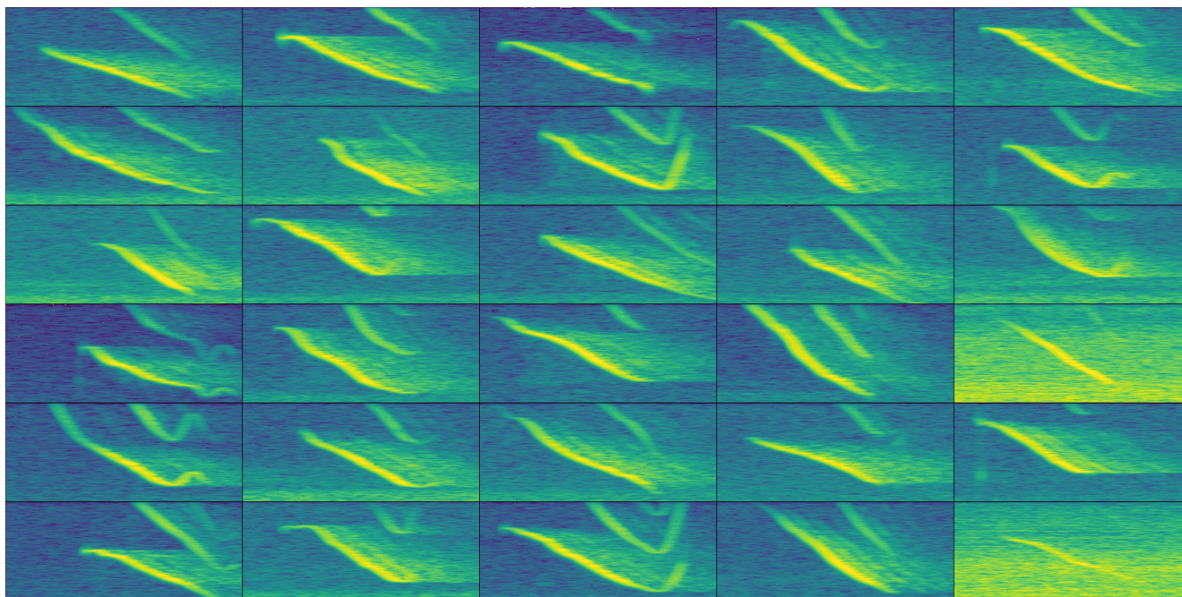
FIGURE 1 Example spectrograms of Spix's disc-winged bats social calls for each of the 30 recordings used in the analysis. The highest signal-to-noise ratio call by sound file are shown. The time scale range is 71 ms and the frequency range 10–44 kHz.
