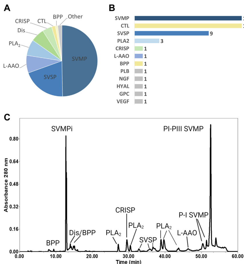
FIG. 2. Crotalus atrox venom proteome characterization. A, toxin family abundances in C. atrox venom modified from Calvete et al. , 2009. B, the number of proteoforms identified in C. atrox venom in the present study organized by family. C, RP-HPLC separated C. atrox venom. For peak identification, fractions were analyzed with mass spectrometry and SDS-PAGE and compared to known masses from Calvete et al. , 2009. PP, bradykinin potentiating peptide; CRISP, cysteine rich secretory protein; CTL, C-type lectin; Dis, disintegrin; GPC, glutaminyl-peptide cyclotransferase; HPLC, high-performance liquid chromatography; HYAL, hyaluronidase; L-AAO, L-amino acid oxidase; NGF, nerve growth factor; PLA 2 , phospholipase A 2 ; PLB, phospholipase B; RP-HPLC, reverse-phase high-performance liquid chromatography; SVMP, snake venom metalloprotease; SVMPi, SVMP tripeptide inhibitor; SVSP, snake venom serine protease; VEGF, vascular endothelial growth factor.
