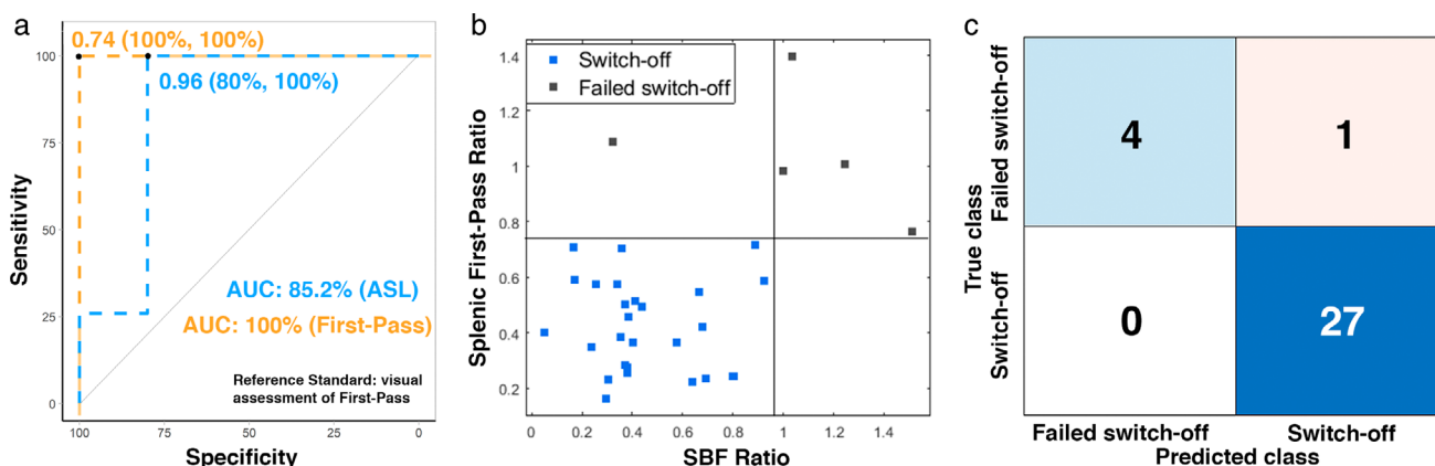
FIGURE 8: Splenic perfusion measurements obtained considering all patients. (a) Receiver-operator characteristic curve curves (in orange for first-pass and in blue for PCASL) for the detection of splenic switch-off. (b) Scatter plot of stress-to-rest ratios, where the vertical and horizontal lines indicate the PCASL and first-pass cut-off values, respectively. (c) Confusion matrix for classification using first-pass as ground truth.
