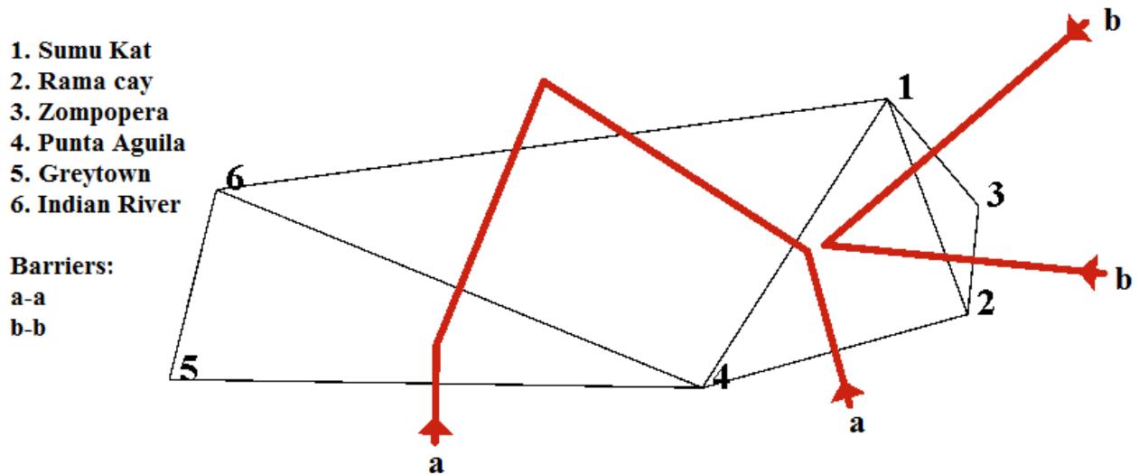
Figure 46. Delaunay triangulation using the Monmonier's algorithm. Thin lines connect Rama localities crossed by barriers of gene flow that are represented by arrows and thick lines.
