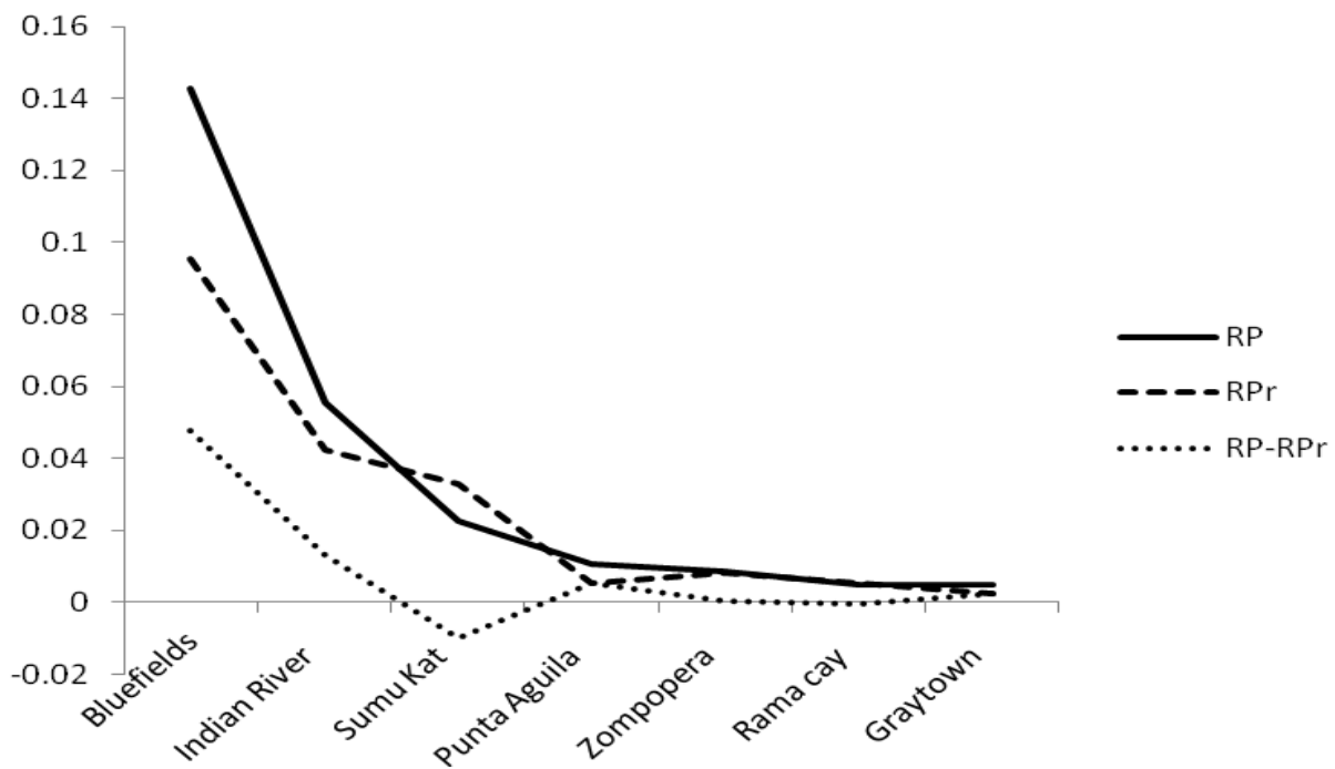
Figure 37. Trends in RP , RP_r , and RP-RPr values. Bluefields, Indian River, and Sumu Kat are the most isolated populations with less internal subdivisions. Punta Aguila and Greytown have the highest degree of internal subdivisions.
