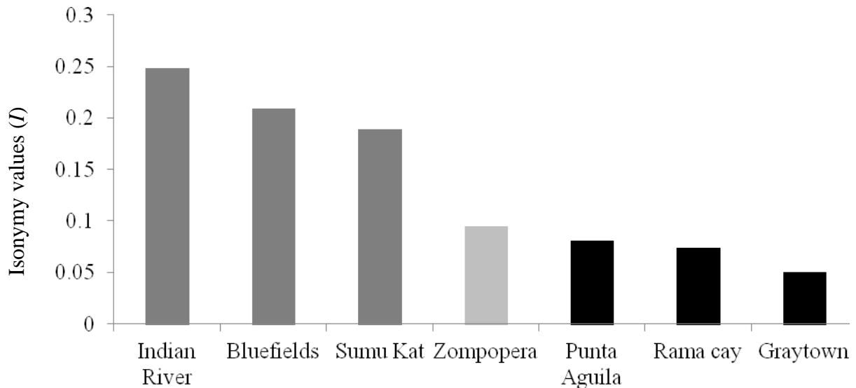
Figure 32. Isonymy values (Y-axis) based on surnames of seven Rama localities (X-axis). Indian River, Bluefields, Sumu Kat, and Zompopera present the highest isolation. Punta Aguila, Rama Cay, and Greytown are the less isolated.
