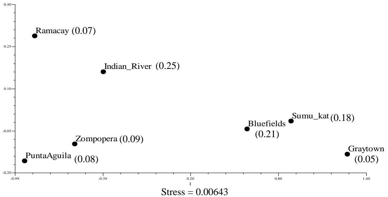
Figure 36. MDS coefficient of kinship between subpopulations ( I_{ij} ) and unbiased Isonymy values in parenthesis ( I_{ij} ).
