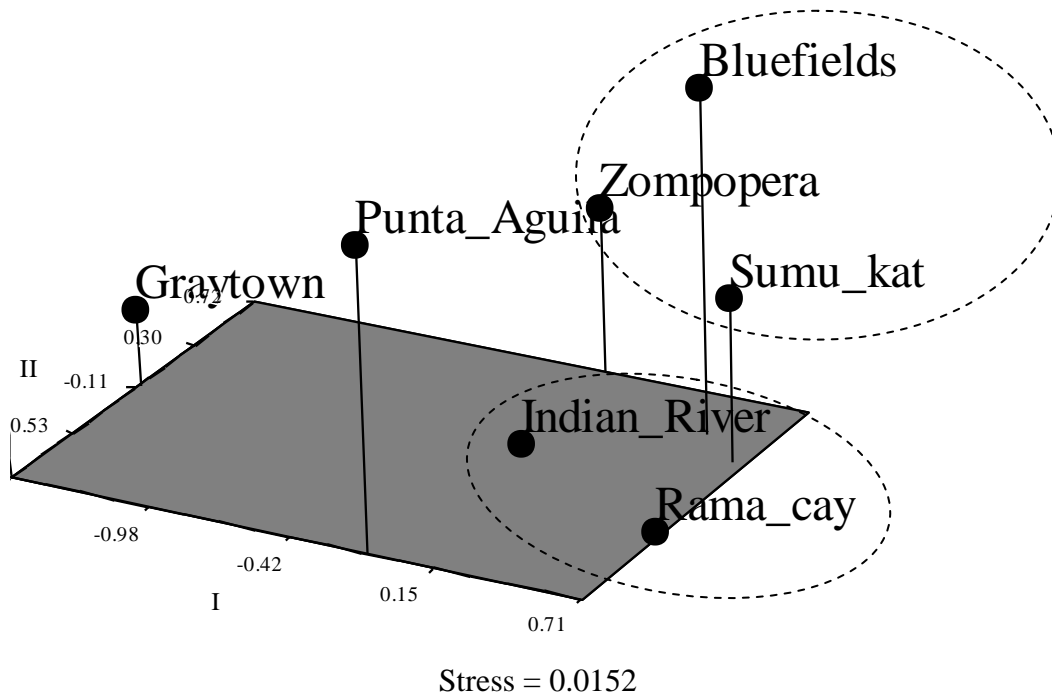
Figure 39. 3-D MDS of Lasker's D showing kinship relationships based on isonymy between populations.
