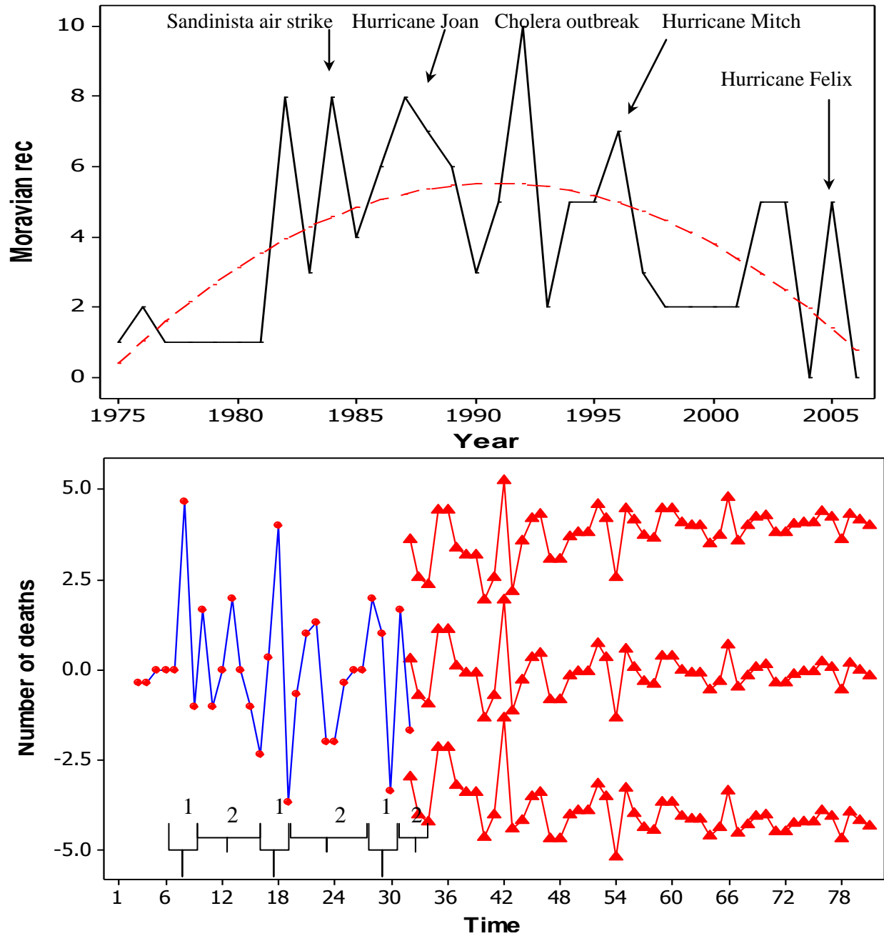
Figure 28. Top graph: secular trend of mortality and fitted quadratic curve ( Death = -0.28 + 0.691 \cdot year - 0.02054 \cdot year^2 , MAPE = 70.8, MAD = 1.8, MSD = 4.6). Lower graph: ARIMA model (0, 0, 1). Number 1 in the graph represents a higher peak in mortality every ~7-8 years; number 2 represents subsequent peaks in mortality every ~ 3 years. Broadcasting represents peaks in mortality patterns if similar environmental conditions are present in the southern Moskitia of Nicaragua.
