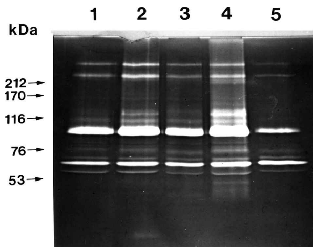
FIG. 1. Zymograms of muscle homogenates from mice injected i.m. with 60 µg of MT-III or BaP1. Gelatinase activity was assessed by sodium dodecyl sulfate-polyacrylamide gel electrophoresis (5–20% acrylamide gradient) containing 1% type A gelatin. Muscle homogenates after injection of: (1) BaP1, 1 h; (2) BaP1, 6 h; (3) MT-III, 1 h; (4) MT-III, 6 h; (5) saline. Molecular weight markers are depicted to the left.
