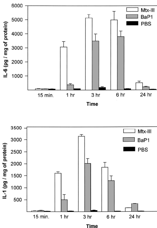
FIG. 2. Increments of IL-1β and IL-6 in muscle homogenates after i.m. injection of 60 µg of MT-III or BaP1, dissolved in 60 µl of saline solution. Control mice received saline solution alone. Mice were injected in the right gastrocnemius and, at various time intervals, they were killed and the injected muscle was excised, weighed and homogenized in 2.0 ml of saline solution. After centrifugation, cytokine levels were quantitated by enzyme-linked immunosorbent assay (see Materials and methods). Results are presented as mean ± standard deviation ( n = 4).
