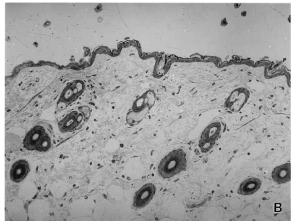
FIG. 3. Light micrographs of sections of skin from mice injected i.m. in the gastrocnemius with 60 \mu\text{g} of either BaP1 (A) or MT-III (B). Tissue samples were obtained 3 h after injection, processed and embedded in Spurr resin. Thick ( 1 \mu\text{m} ) sections were stained with toluidine blue. Notice the presence of hemorrhage in the dermis and the formation of a blister (Bli) in mice injected with BaP1, whereas no evident pathological alterations in dermis and epidermis were observed after injection of MT-III.
